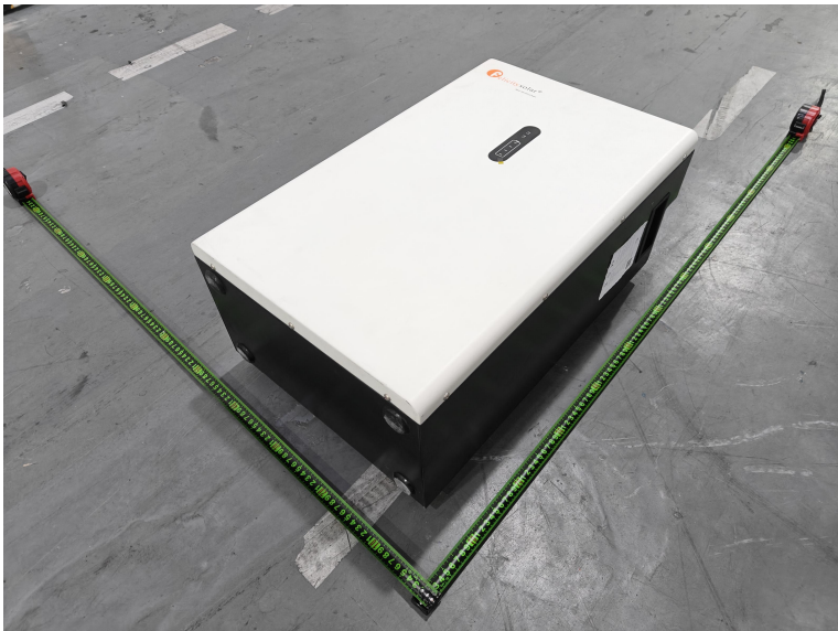
Battery: LPBA48200WG1, 51.2V, 200Ah, 10.24kWh
