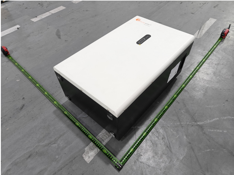
Battery: LPBA48200WG1, 51.2V, 200Ah, 10.24kWh
