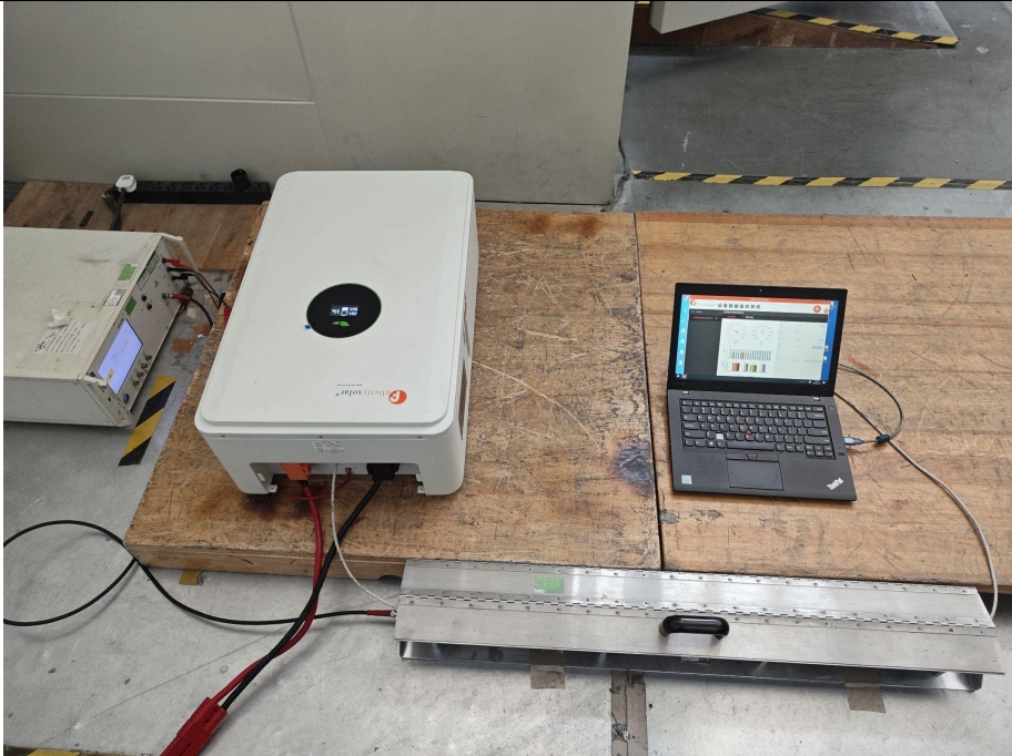
Set-up for Radio-Frequency Electromagnetic Field
