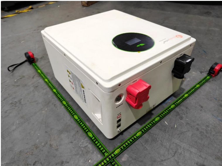
Battery: FLA24300WG2, 25.6V, 300Ah, 7.5kWh
