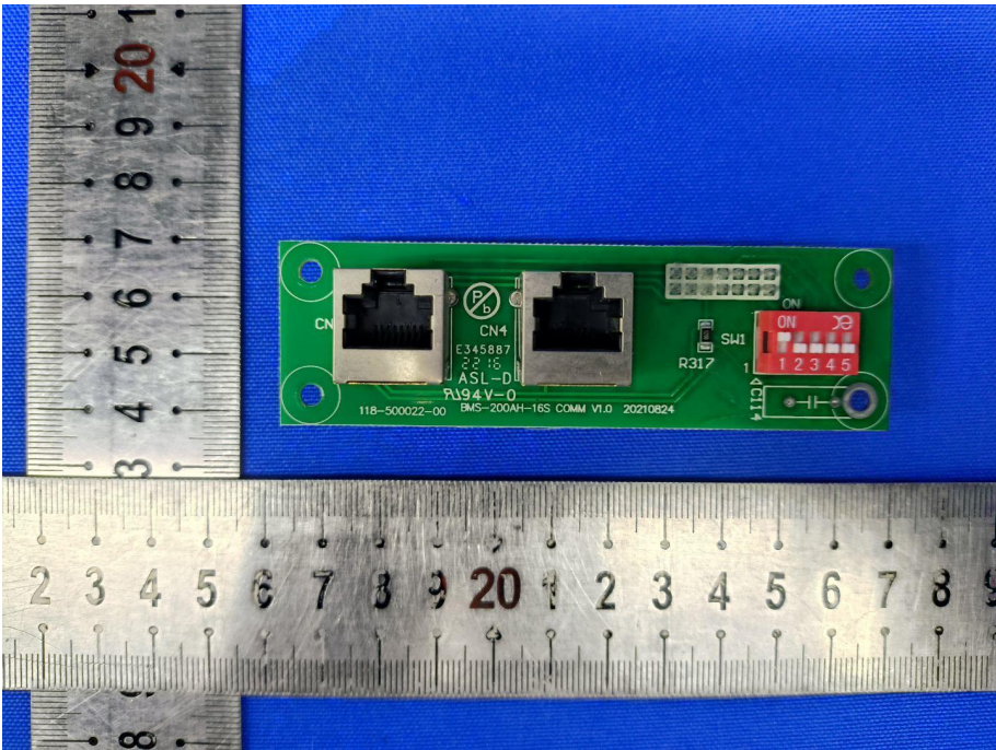
PCB View -1
