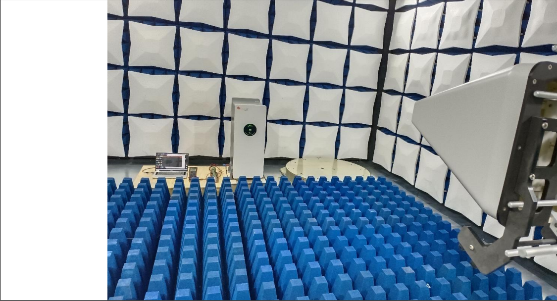
Set-up for Radio-Frequency Electromagnetic Field
