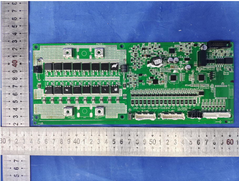
PCB View -1
