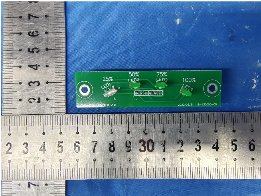
PCB View -3
