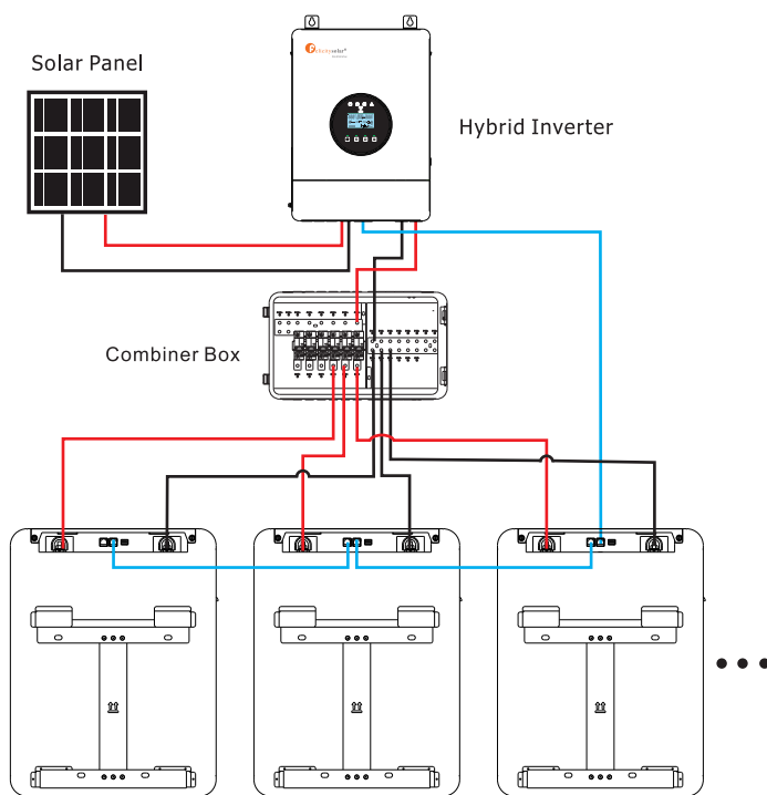
Figure 3-2 Multiple Battery Parallel System Connection Diagram
