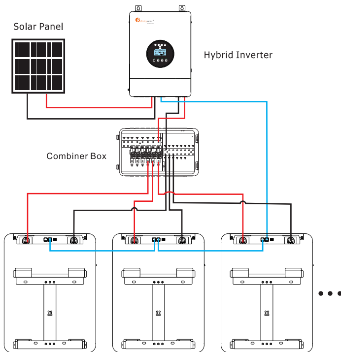
Figure 4-1 The parallel connection of three battery packs
