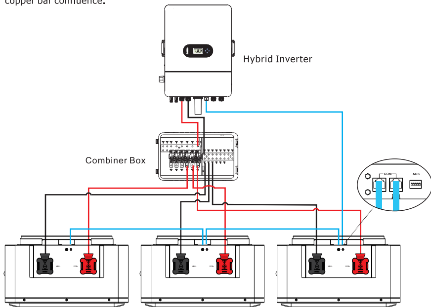
Figure 4-1 The parallel connection of three battery packs
