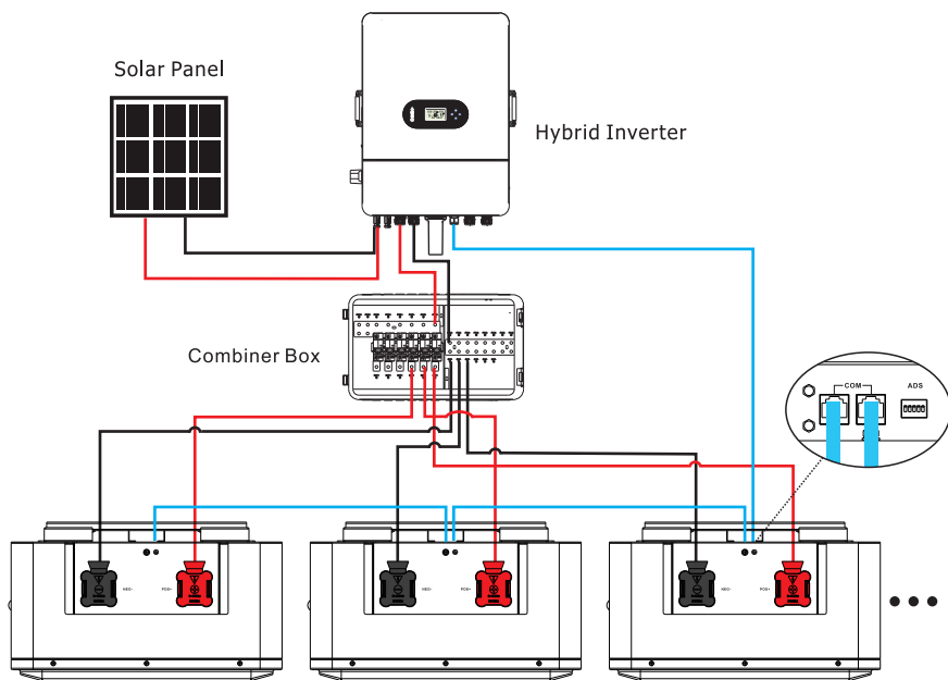
Figure 3-2 Multiple Battery Parallel System Connection Diagram
