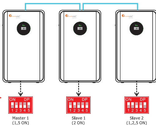
Example of three batteries in parallel
