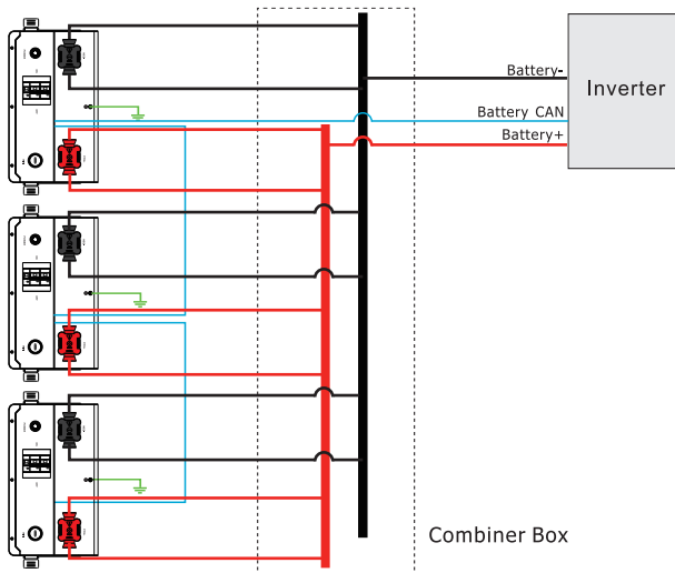
Figure 4-1 The parallel connection of three battery packs
