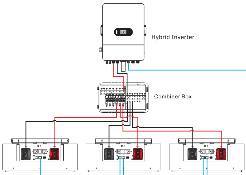
Figure 4-1 The parallel connection of three battery packs
