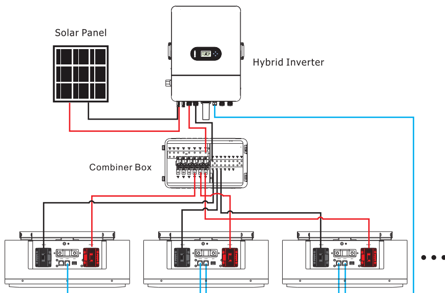
Figure 3-2 Multiple Battery Parallel System Connection Diagram
