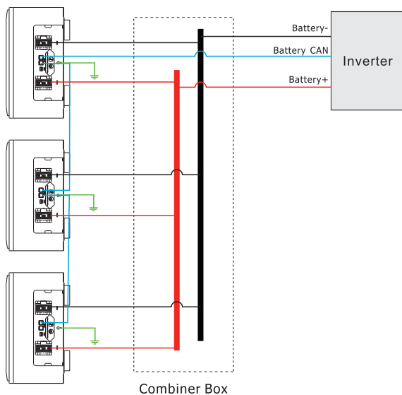
Figure 4-1 The parallel connection of three battery packs
