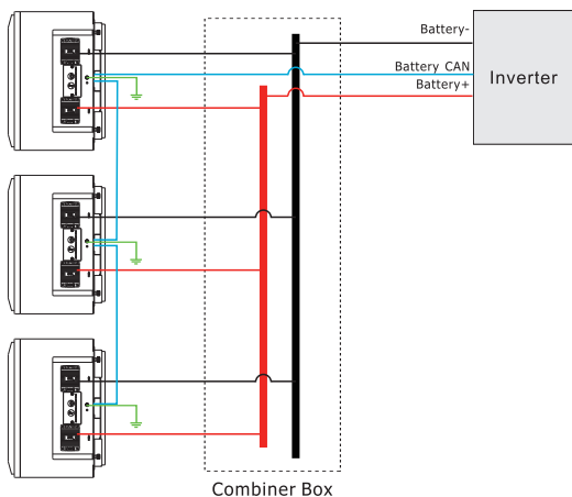
Figure 4-1 The parallel connection of three battery packs
