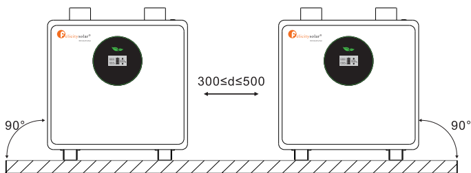
Ground(Two rows installation)
