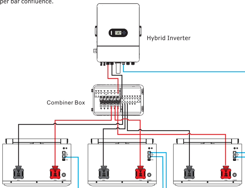
Figure 4-1 The parallel connection of three battery packs
