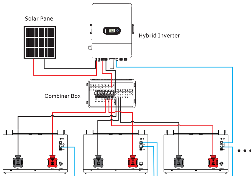
Figure 3-2 Multiple Battery Parallel System Connection Diagram
