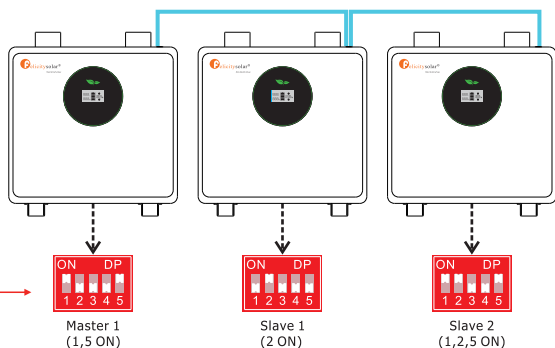
Example of three batteries in parallel
