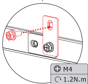
Step 3. Install the screws
