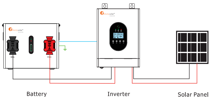
Figure 3-1 Single Battery System Connection Diagram
