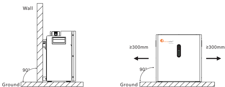
Ground(Two rows installtion)
