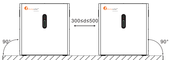
Ground(Two rows installtion)
