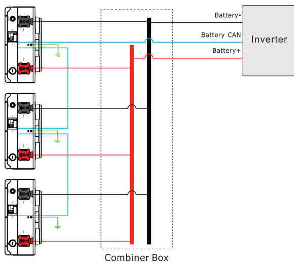
Figure 4-1 The parallel connection of three battery packs
